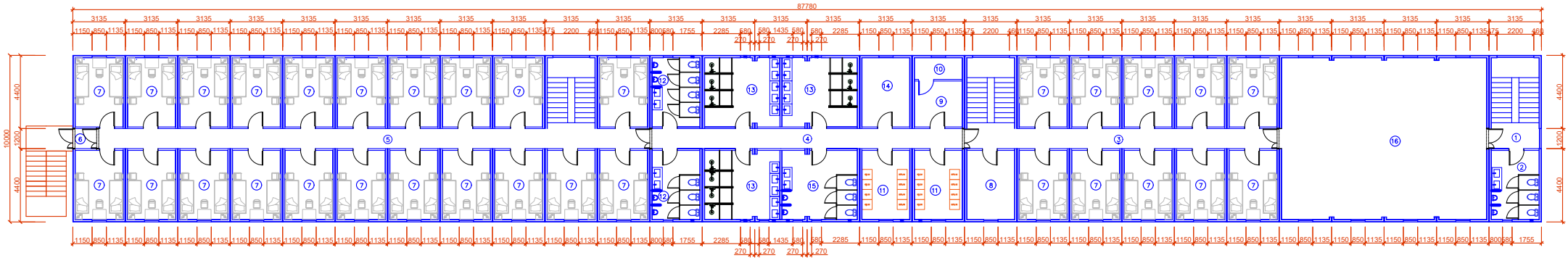
3rd Floor Layout 38 rooms - 152 beds
