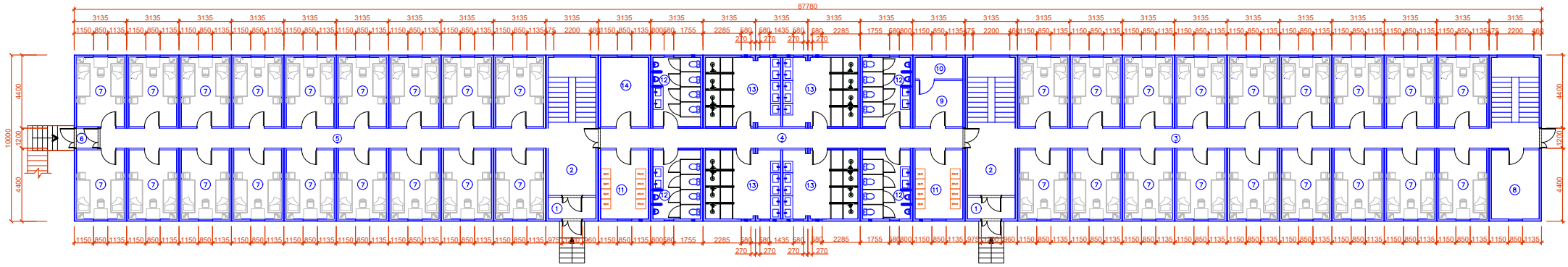
2nd Floor Layout 30 rooms - 120 beds
